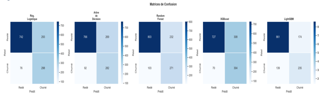
Figure 13. Matrices de confusion comparatives.
